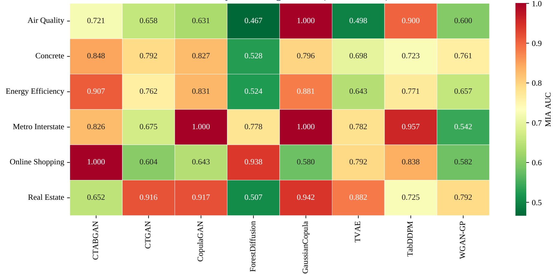
MIA AUC by dataset × generator (10-seed mean)
